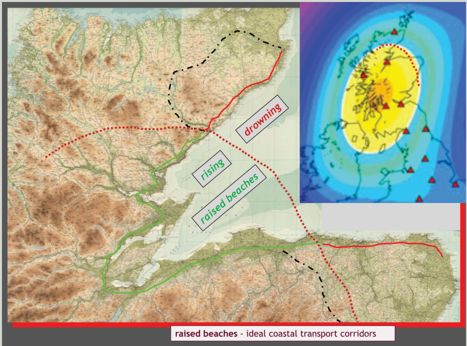
The 'hinge line' intersecting the Moray Firth coasts at Helmsdale and Cullen (inset - most of Scotland is still bouncing back - yellow oval). Most of the green coastline has raised beaches; most of the red is cliffed. Black dashes – Far North and Aberdeen lines forced inland to avoid coastal cliffs.
